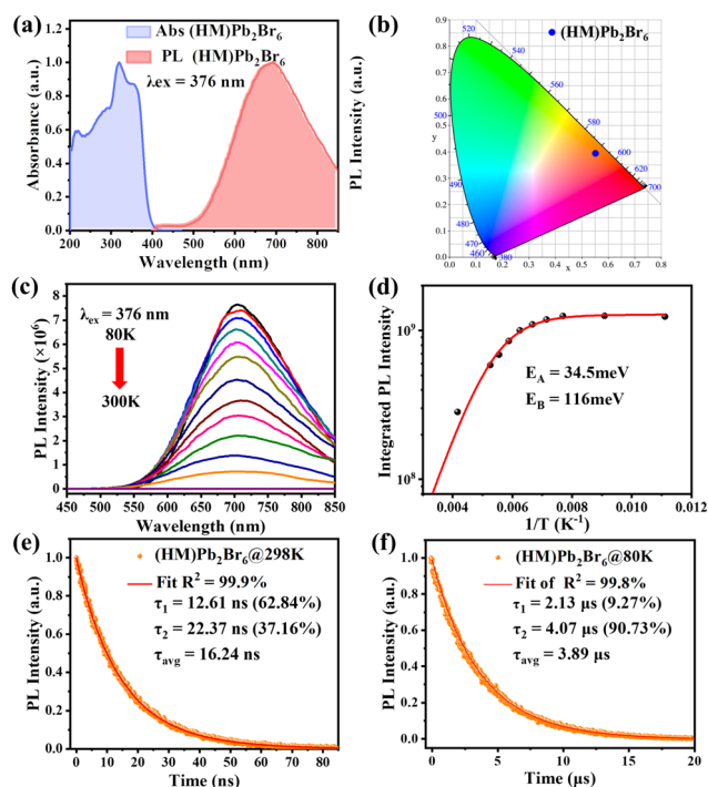
Fig. 2 (a) Normalized absorption and PL spectra of (\text{HM})\text{Pb}_2\text{Br}_6 . (b) The CIE 1931 chromaticity coordinate. (c) Temperature-dependent PL spectra of (\text{HM})\text{Pb}_2\text{Br}_6 . (d) Integrated PL intensity as a function of reciprocal temperature. Time-resolved PL decay curve of (\text{HM})\text{Pb}_2\text{Br}_6 under a 375 nm excitation laser line at (e) 298 K and (f) 80 K.
