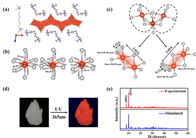
Fig. 1 (a) Crystal structure of (\text{HM})\text{Pb}_2\text{Br}_6 . (b) The Pb–Br bond lengths and Br–Pb–Br bond angles of three individual polyhedra. (c) The detailed view of the Pb–Pb and Br–Br pair distance determined from the SCXRD analysis. (d) Photographs of (\text{HM})\text{Pb}_2\text{Br}_6 single crystals under ambient light (left) and UV 365 nm light (right). (e) The experimental and simulated XRD patterns of (\text{HM})\text{Pb}_2\text{Br}_6 .
