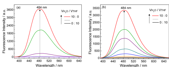
Fig. 4 Fluorescence spectra of (a) L -1 and (b) \text{Ag}^+-\text{L}-1 in \text{H}_2\text{O}/\text{THF} mixtures with increasing volume fractions of \text{H}_2\text{O} . \lambda_{\text{ex}} = 350 \text{ nm} , [\text{L}-1] = [\text{Ag}^+-\text{L}-1] = 25 \mu\text{M} .
