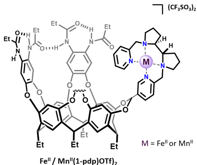
Fig. 1 Representation of cavitant-tailored bioinspired complexes Fe II ( 1-pdp )(OTf) 2 and Mn II ( 1-pdp )(OTf) 2 .
