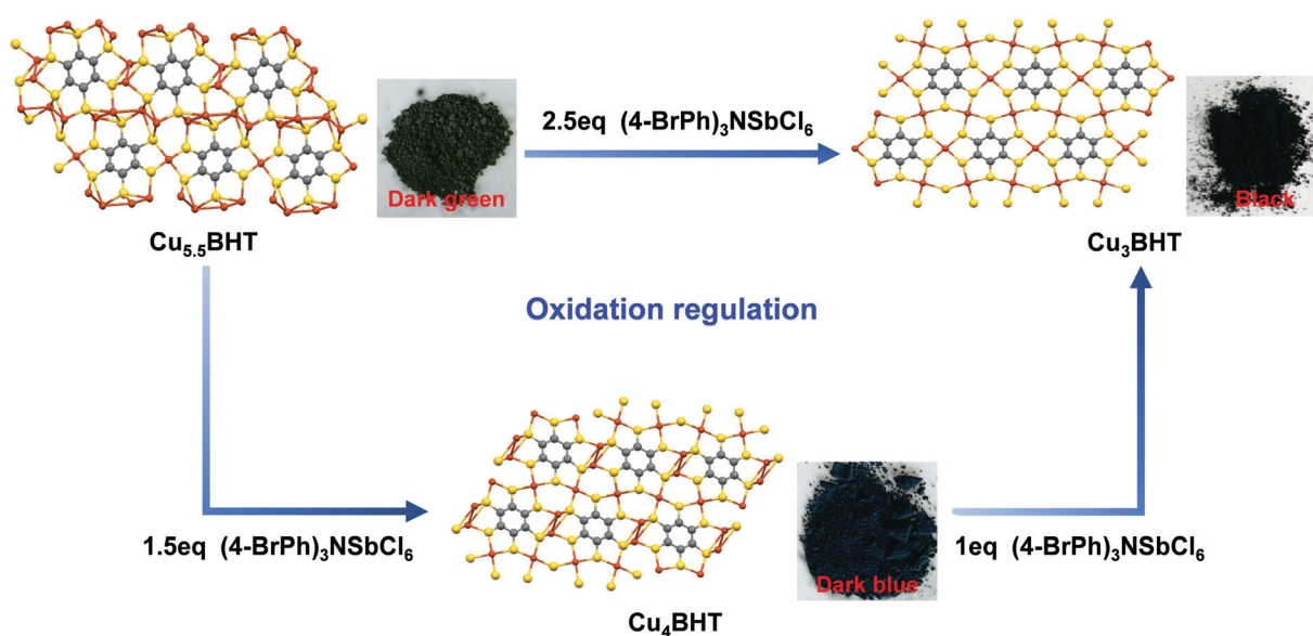
Fig. 5 Oxidation regulation within the \text{Cu}_x\text{BHT} family. Schematic illustration of phase transition in \text{Cu}_x\text{BHT} species upon delicate oxidation regulation with (4\text{-BrPh})_3\text{NSbCl}_6 . Photograph shows the colours of each \text{Cu}_x\text{BHT} species.
