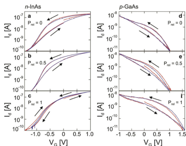
Fig. 13 The transfer characteristics for transistors based upon semiconductor nanowires and a PEO top gate (wire type indicated). P rel indicates the relative water vapour pressure ( i.e. relative humidity). Reprinted with permission from D. J. Carrad et al. Nano Lett. , 2017, 17 , 827–833. Copyright 2017 American Chemical Society. 81
