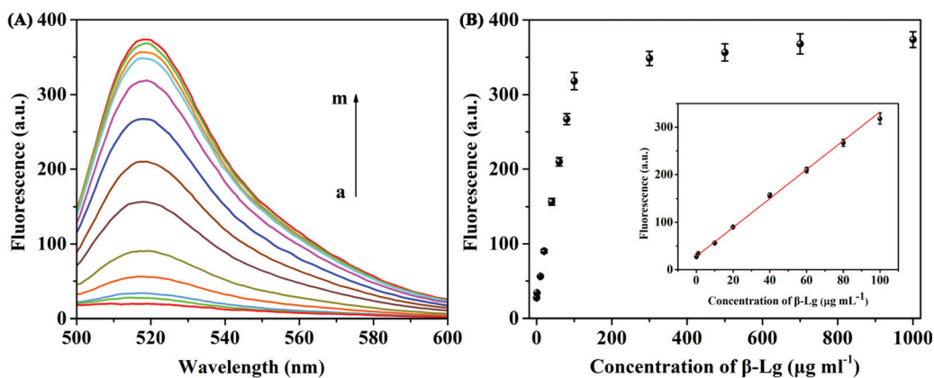
Fig. 4 (A) FAM labelled \beta -Lg aptamer fluorescence emission spectra of the proposed method at different concentrations of \beta -Lg ( 0, 0.1, 1, 10, 20, 40, 60, 80, 100, 300, 500, 700, \text{ and } 1000 \mu\text{g mL}^{-1} ). (B) Diagram of peak fluorescence and target \beta -Lg concentration. Inset: Linear fitting of fluorescence intensity at 518 nm with the target \beta -Lg concentration.
