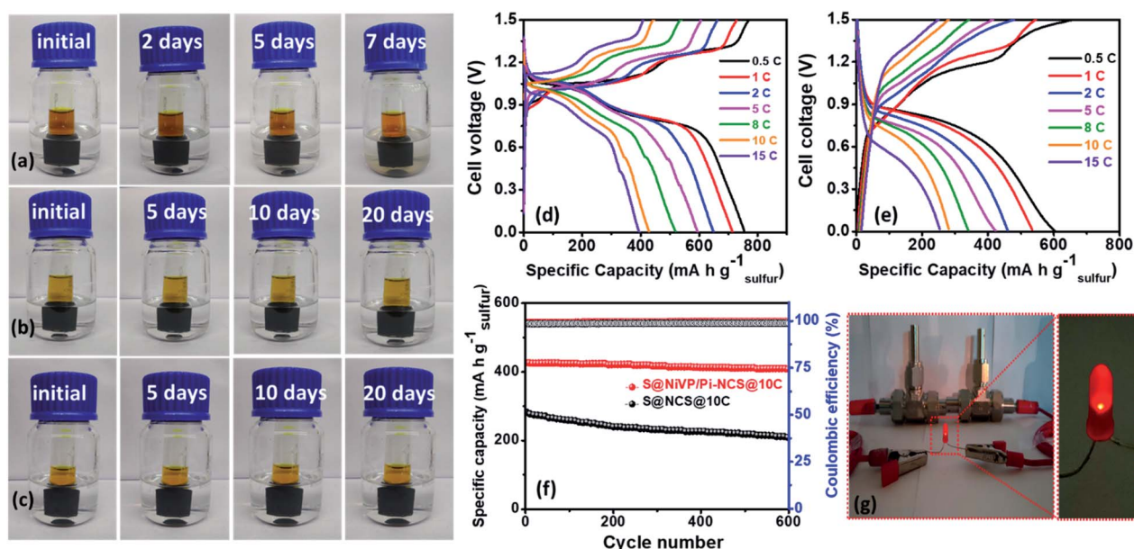
Fig. 5 Nafion membrane polysulfide leakage test with different salt concentrations after variable resting times: (a) 2 M polysulfide dissolved in a 2 M \text{Na}_2\text{SO}_4 aqueous electrolyte in a small vial and then inverted into 2 M \text{Na}_2\text{SO}_4 in water, (b) 1 M polysulfide dissolved in a 2 M \text{Na}_2\text{SO}_4 aqueous electrolyte and then placed in 2 M \text{Na}_2\text{SO}_4 in water, (c) 0.5 M polysulfide dissolved in a 2 M \text{Na}_2\text{SO}_4 aqueous electrolyte and then placed in a 2 M \text{Na}_2\text{SO}_4 in water, galvanostatic charge–discharge curves of full cell battery assembled using Nafion membrane with (d) \text{S@NiVP/Pi-NCS} anode + \text{Na}_{0.44}\text{MnO}_2 cathode and (e) \text{S@NCS} anode + \text{Na}_{0.44}\text{MnO}_2 cathode at various C-rates, (f) corresponding battery cycling performances and coulombic efficiency at 10C respectively over 600 cycles in 2 M aq. \text{Na}_2\text{SO}_4 , (g) demonstration of two aqueous Na-ion/S battery consisting of \text{S@NiVP/Pi-NCS} anode and \text{Na}_{0.44}\text{MnO}_2 cathode powering LED.
