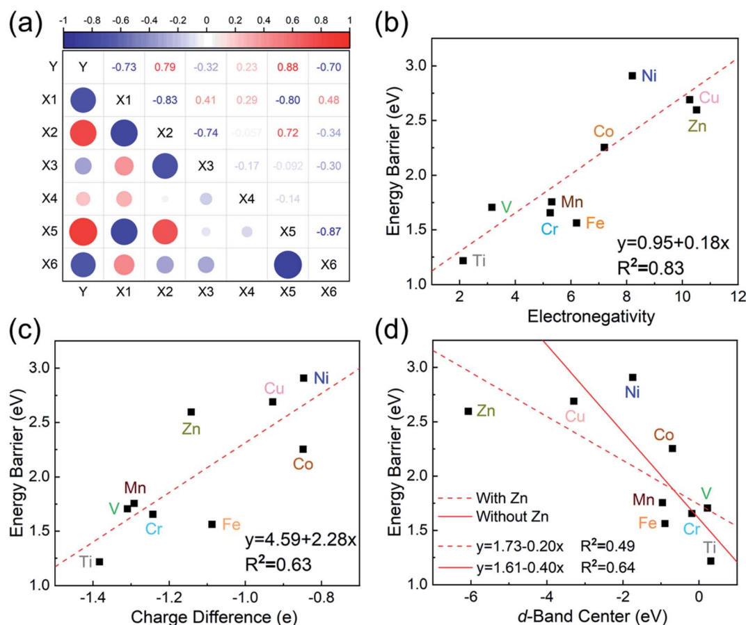
Fig. 3 (a) Correlation matrix of PCCs between material properties and the dehydrogenation energy barriers of MgH 2 upon addition of SACs. Y is energy barrier, X 1 is the height of metal atoms, X 2 is the difference in the charge of metal atoms, X 3 is the difference in the charge of N, X 4 is H adsorption energy, X 5 is electronegativity, and X 6 is the d-band center. The value domain of PCCs is [-1,1]. The size of the circle represents the size of its corresponding PCC values. Blue and red indicate positive and negative correlations, respectively. (b–d) Correlations of (b) electronegativity vs. energy barrier, (c) metal charge difference vs. energy barrier, and (d) metal d-band center vs. energy barrier. The red dotted line represents the fitted curve with all data, while the red solid line represents the fitted curve without the outlier SACs–Zn.
