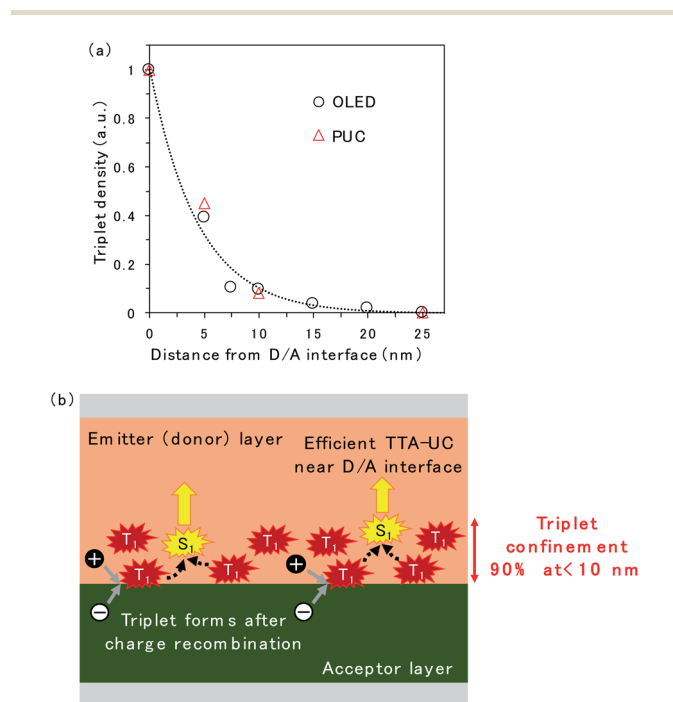
Fig. 5 (a) Relative triplet density as a function of distance from the D/A interface. The relative triplet density was calculated according to the intensity change of EL and PUC emission from rubrene when a CuPc-doped layer was inserted at the D/A interface. The black circle represents triplet density in the rubrene/PTCDI OLED device, while the red triangle represents triplet density in the rubrene/ITIC-Cl PUC system. The broken line denotes fitting done using the single exponential regarding the OLED device. (b) Schematic of triplet exciton accumulation after charge recombination near the D/A interface.
