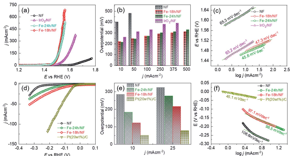
Fig. 4 Comparison of the electrocatalytic performance of the etched NFs and a benchmark catalyst in a 1 M KOH solution: (a) iR compensated anodic LSVs for the pristine NF, etched NF, and benchmark \text{IrO}_2/\text{NF} electrodes, (b) overpotential profiles with respect to the OER current density, and (c) corresponding Tafel slopes extracted from the LSVs. (d) iR compensated cathodic LSVs of the pristine NF, etched NFs, and benchmark \text{Pt}(20\text{wt}\%)/\text{C}/\text{NF} electrodes, (e) overpotential profiles with respect to the HER current density, and (f) corresponding Tafel slopes extracted from the LSVs.
