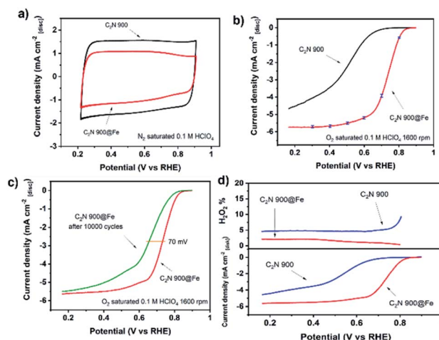
Fig. 4 Cyclic voltammogram of C_2N\ 900 before and after Fe metalation recorded at 50\ mV\ s^{-1} (a). Capacitance-corrected cathodic scan of the cyclic voltammogram in 0.1 M HClO_4 with a rotation speed of 1600 rpm recorded at 10\ mV\ s^{-1} obtained by subtracting N_2 saturated cyclic voltammetry at 1600 rpm from the O_2 saturated result. For C_2N\ 900@Fe , three independent measurements were carried out with average value plotted. Error bars correspond to largest deviating value from average at the given potential. (b). Cathodic scans of the cyclic voltammograms at 1600 rpm before and after 10 000 cycles between 0.6 and 0.9 V recorded at 100\ mV\ s^{-1} under N_2 saturation (c). H_2O_2 production from cathodic scan RRDE measurement for C_2N\ 900 and C_2N\ 900@Fe at 1600 rpm, 10\ mV\ s^{-1} , capacitance correction and under O_2 saturation (d). All measurements conducted with no IR correction, 0.26\ mg\ cm^{-2} catalyst loading and room temperature electrolyte.
