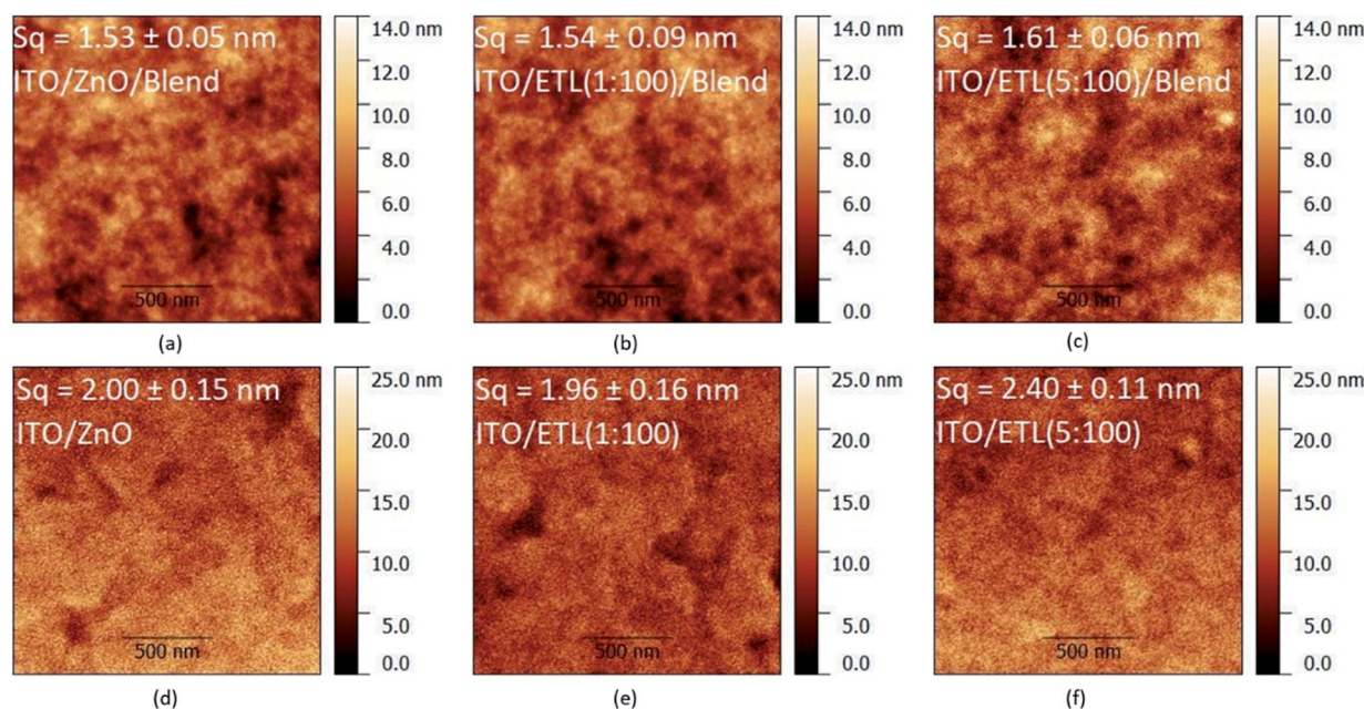
Fig. 2 Tapping mode AFM images (1.6 μm × 1.6 μm, annotated with the corresponding root mean square roughness (Sq)) of the topography of (a) ITO/ZnO/PTB7-Th : PC 70 BM, (b) ITO/Mg-doped (1 : 100) ZnO/PTB7-Th : PC 70 BM, (c) ITO/Mg-doped (5 : 100) ZnO/PTB7-Th : PC 70 BM, (d) ITO/ZnO, (e) ITO/Mg-doped (1 : 100) ZnO and (f) ITO/Mg-doped (5 : 100) ZnO. There is no significant variation of Sq between the bare ITO/ZnO and ITO/Mg-doped (1 : 100) ZnO films, although Sq is ≈ 20% larger for the (5 : 100) MgO : ZnO films. Mg-doping of the ETL does not influence the morphology of the PTB7-Th : PC 70 BM blend for the investigated length scales.
