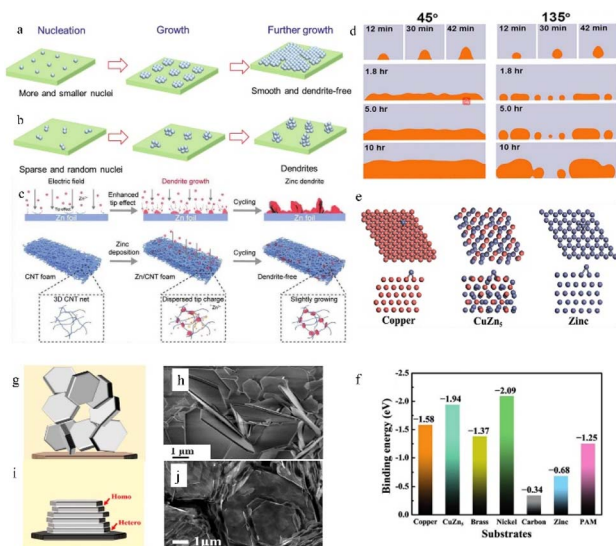
Fig. 5 Schematic illustration of the Zn deposition process. (a) A uniform and dendrite-free zinc morphology is enabled by more and smaller nuclei. (b) Zn dendrites develop when there are few and random nuclei. Adapted from ref. 40. Copyright 2022, Wiley-VCH GmbH. (c) Effect of the 3D structure on zinc deposition. Adapted from ref. 64. Copyright 2022, Wiley-VCH GmbH. (d) Effect of the initial wetting angles on the following deposition process. Adapted from ref. 66. Copyright 2014, Elsevier Ltd. (e) The models of the affinity between different substrates and zinc. (f) Calculated binding energies between different substrates and zinc. Adapted from ref. 62. Copyright 2019, Wiley-VCH GmbH. (g) The epitaxial electrodeposition of Zn metal. (h) Morphology of zinc deposits on stainless steel. (i) Illustration of the uneven electrodeposition of Zn. (j) Morphology of zinc deposits on graphene-coated stainless steel. Adapted from ref. 68. Copyright 2019, AAAS.
