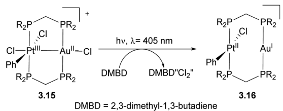
Scheme 19 The reactivity of Pt/Au complexes in halogen photoelmination.
