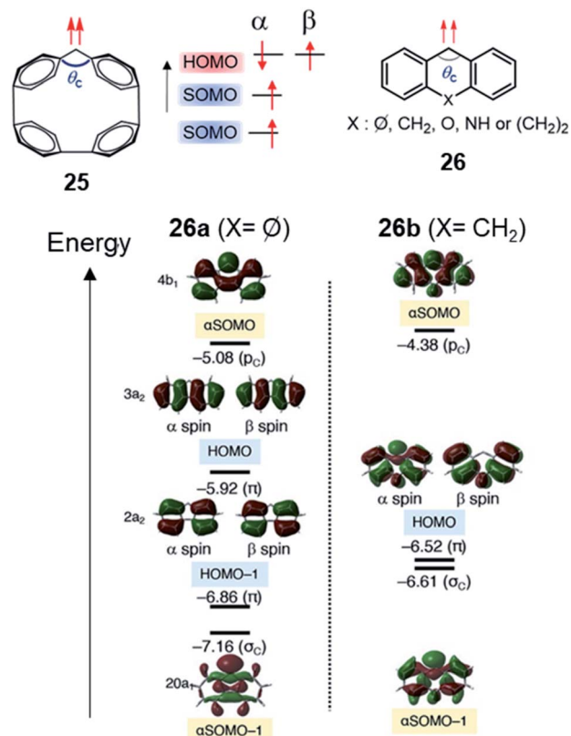
Fig. 17 Top: triplet carbenes included in a cycloparaphenylene (CPP) scaffold 25 and 2,2-difluorocyclopentane diradical 26 (left) showing SHI; with corresponding molecular orbital diagrams for 26a and 26b . Figure reprinted with permission from ref. 54. Copyright 2021 by the American Chemical Society.
