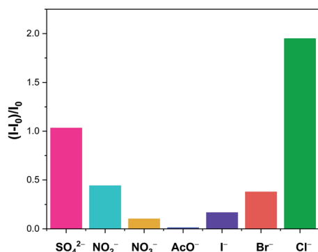
Fig. 10 Relative emission intensity increase of 10\ \mu\text{M} tetraphenylethene AIE anion sensor 5.XB in the presence of 10 equiv. of various anions in THF. Reproduced from ref. 100 under the terms of the CC BY license.
