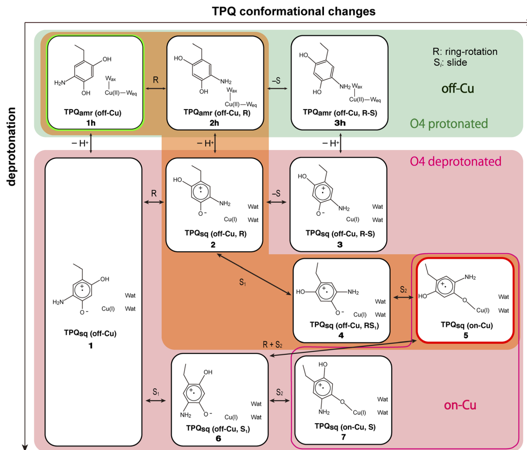
Fig. 4 A comprehensive view of the intermediate states on which the present work is focused for the TPQ amr to TPQ sq transition. The letter "h" added in the labeling as in 1 h –3 h stands for the protonated state on O4-TPQ. The orange background highlights the main reaction pathway, whereas the green background refers to the O4-TPQ protonated state, and the red one refers to the deprotonated one.
