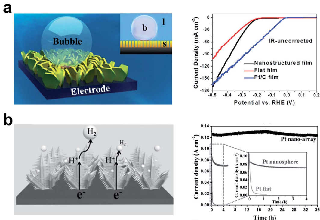
Fig. 7 The highly efficient HER on an underwater superhydrophobic electrode. (a) Schematic of the adhesion behavior of bubbles on the superhydrophobic electrode (left). The superhydrophobic electrode (nanostructured film) showed high HER performance compared with flat films and Pt/C films, (right). Adapted from ref. 92 with permission. Copyright 2014, Wiley-VCH. (b) The pine-shaped Pt nanoarray superhydrophobic electrode for the HER (left). Pine-shaped Pt nanoarray superhydrophobic electrode showed good long-term stability compared with the Pt nanosphere electrode and the Pt flat electrode (right). Adapted from ref. 119 with permission. Copyright 2015, Wiley-VCH.
