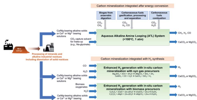
Fig. 5 Conceptual solvent-based capture and concurrent mineralization. Image from Gadikota et al. , 2021. 100
