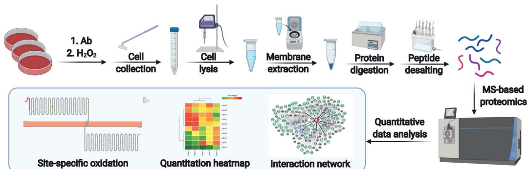
Fig. 1 Workflows of AAPT method. (a) Workflows of antibody modification with two approaches including FeDBAb and FeAb. (b) The details of the treatment of cells with modified antibodies and H_2O_2 . Cells are treated with modified antibodies followed by H_2O_2 treatment. Proteins in close proximity to the reaction are specifically oxidized. (c) The workflow of sample preparation, data acquisition, and data analysis.
