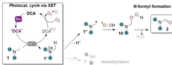
Fig. 5 SET reductive quenching mechanism of DCA proposed by Santamaria and co-workers leading to demethylation and N -formyl products.
