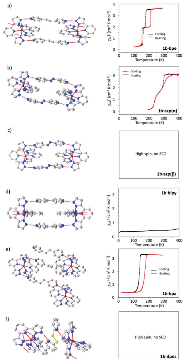
Fig. 5 Fragments of the crystal structures of each coformer of 1b (left) and curves indicating their SCO behaviour (right). (a) AB-type 1D chain structure observed in 1b·bpe at 200 K (on cooling). (b) AB-type 1D chain structure of 1b·azp(α) at 270 K. (c) CC-type 1D chain structure of 1b·azp(β) at 250 K. (d) AB-type 1D chain structure observed in 1b·bipy at 298 K. (e) 2D supramolecular sheet structure of 1b·bpa at 190 K. (f) 3D supramolecular network structure of 1b·dpds at 80 K. Atomic displacement parameters are drawn at 50% probability.
