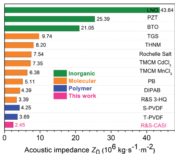
Fig. 8 Acoustic impedance characteristics of ( R and S )-CSAI compared with those of some inorganic, polymer, and molecular ferroelectrics. \text{LiNbO}_3 (LNO), \text{Pb}(\text{Zr}_{0.52}\text{Ti}_{0.48})\text{O}_3 (PZT), \text{BaTiO}_3 (BTO), triglycine sulfate (TGS), tris(hydroxymethyl)nitromethane (THNM), 37 trimethylchloromethylammonium cadmium trichloride (TMCMCdCl 3 ), 29 trimethylchloromethylammonium manganese trichloride (TMCM MnCl 3 ), 29 phenylammonium bromide (PB), 20 diisopropylammonium bromide (DIPAB), 16 ( R and S )-3-hydroxyquinoline (R&S-3-HQ), 36 poly(vinylidene fluoride) standard ( S -PVDF), and poly(vinylidene fluoride) thermal pressed ( T -PVDF).
