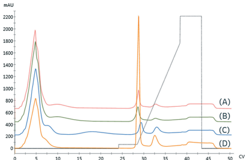
Fig. 5 Initial resin screen for galactose oxidase using 0.5 mL columns with the following resins: (A) GE Ni Sepharose 6FF (B) Ni-NTA Superflow (C) Nuvia IMAC – Ni (D) Nuvia IMAC – Cu. Gradient profile is shown by dashed lines.
