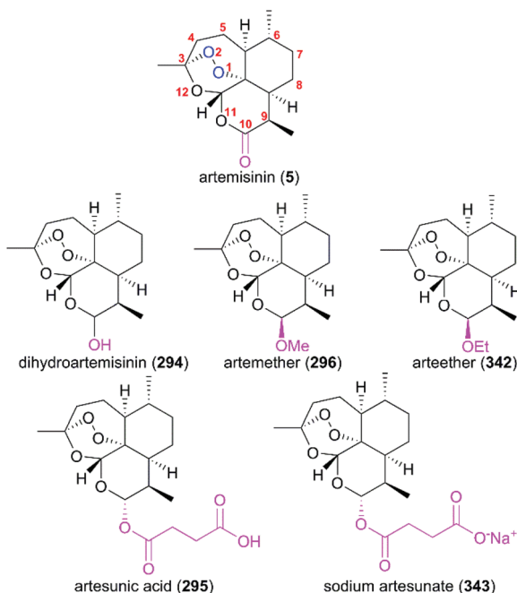
Fig. 14 The first-generation artemisinin derivatives.
