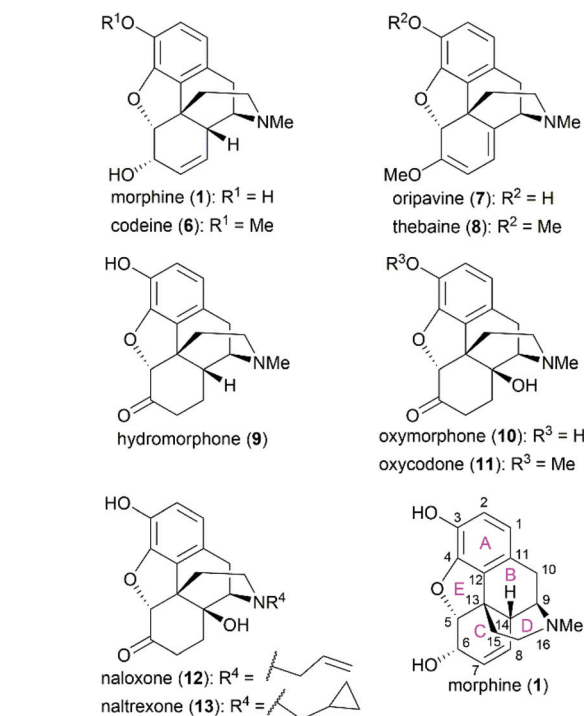
Fig. 2 Morphine and related compounds, and their ring lettering and carbon numbering system.
