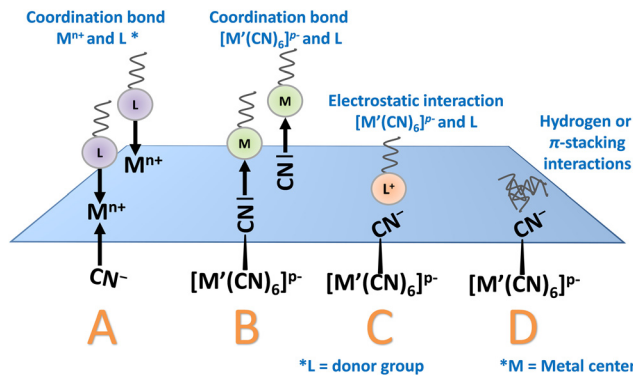
Fig. 5 Schematic representation of different interactions between ligands and PB/PBA nanoparticles: (A) coordination bond between M^{n+} ions and donor group (L); (B) coordination bond between [M'(CN)_6]^{p-} and M; (C) electrostatic interaction between [M'(CN)_6]^{p-} and L; (D) hydrogen or \pi -stacking interactions between cyano-groups and ligands.
