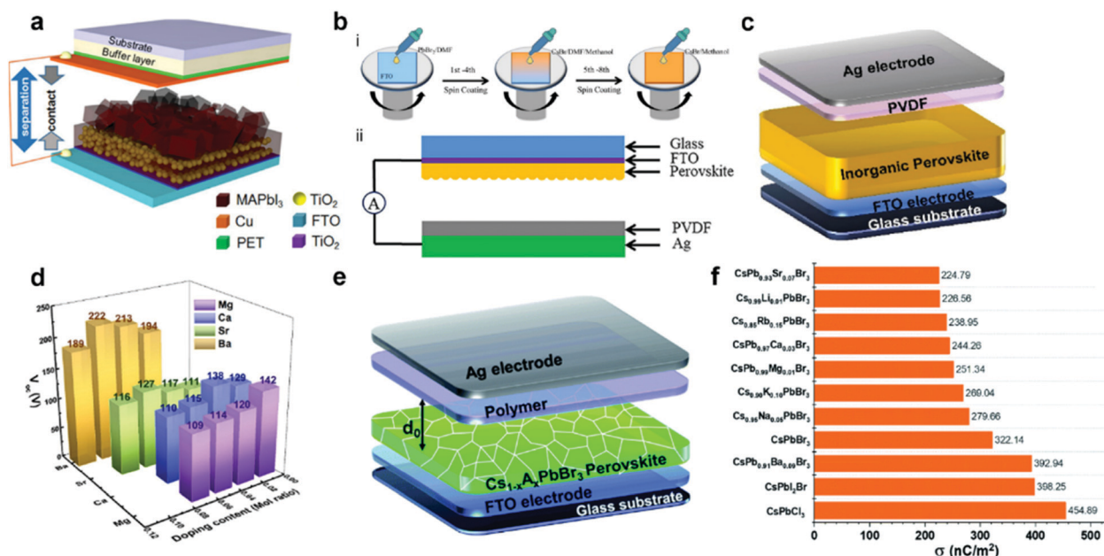
Fig. 6 Device structures of different HP-TENGs and a summary of the triboelectric charge density of inorganic halide perovskites with different ion doping. (a) Device structure of the \text{MAPbI}_3 -based self-powered photodetector. Reproduced with permission from ref. 84. Copyright 2015, American Chemical Society. (b) Schematic illustration of (i) the fabrication process of \text{CsPbBr}_3 thin films using a solvent-etching assisted spin-coating deposition method and (ii) \text{CsPbBr}_3 -based TENG structure. Reproduced with permission from ref. 86. Copyright 2020, Elsevier. (c) Device structure of \text{Ba}^{2+} doped \text{CsPbBr}_3 -based TENG. Reproduced with permission from ref. 89. Copyright 2020, Elsevier. (d) The open-circuit voltage of HP-TENG based on \text{CsPb}_{1-x}\text{M}_x\text{Br}_3 ( \text{M} = \text{Mg}^{2+}, \text{Ca}^{2+}, \text{Sr}^{2+} and \text{Ba}^{2+} , x = 0-1 ) with different doping contents. Reproduced with permission from ref. 87. Copyright 2020, Elsevier. (e) Device structure of \text{Cs}_{1-x}\text{A}_x\text{PbBr}_3 ( \text{A} = \text{Li}^+, \text{Na}^+, \text{K}^+ and \text{Ru}^+ , x = 0-1 )-based TENG. (f) Summary of the triboelectric charge density of inorganic halide perovskites with different ion doping. Reproduced with permission from ref. 90. Copyright 2020, Royal Society of Chemistry.
