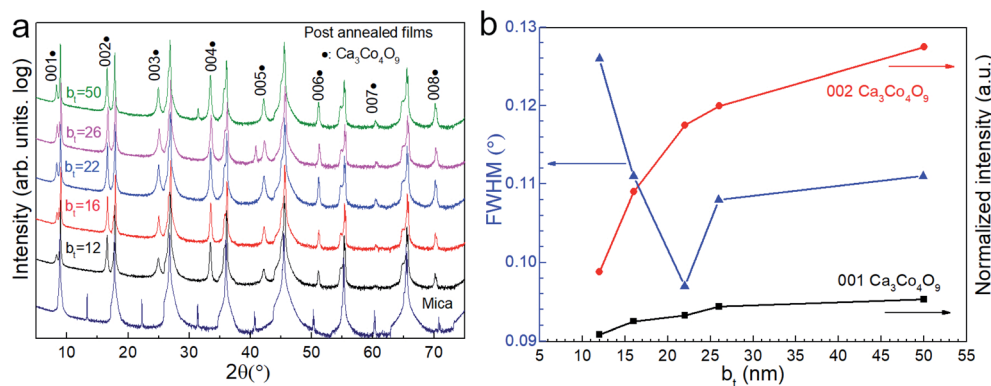
Fig. 4 (a) X-ray diffractograms showing \text{Ca}_3\text{Co}_4\text{O}_9 formation on mica (001) substrate by annealing \text{Ca(OH)}_2/\text{Co}_3\text{O}_4 multilayers with different bilayer thicknesses in the 12 \leq b_t \leq 50 nm range. (b) \text{Ca}_3\text{Co}_4\text{O}_9 001 and 002 peak intensities normalized with the intensity of the corresponding substrate peaks, plotted as a function of b_t .
