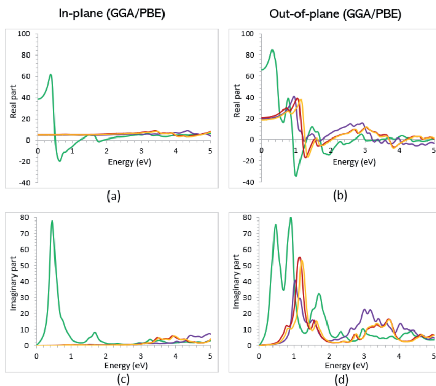
Fig. 4 Imaginary and real parts of the dielectric function of VO 2 (B) PP (green), VO 2 (B) LP (purple), VO 2 (B) PPD (red), and VO 2 (B) LDP (orange) structures along the in-plane (a and c) and out-of-plane (b and d) polarizations, as predicted by RPA + PBE.
