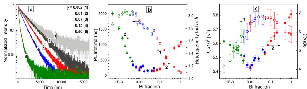
Fig. 7 (a) Kinetic curves of PL decay of CANBIC perovskites with Bi fraction \gamma = 0.002 (curve 1), 0.01 (2), 0.07 (3), 0.15 (4), and 0.50 (5). Dashed lines represent the fitting of the experimental curves with a stretched exponential function. (b) PL lifetime (hollow scatters 1) and heterogeneity factor h (filled scatters 2) derived as functions of \gamma . (c) Rate constants of radiative recombination k_r (hollow scatters 1) and non-radiative recombination k_{nr} (filled scatters 2) as functions of \gamma . Shape of scatters indicates the range of Bi content variation: 0.1 (squares), 0.005–0.05 (circles), and 0.0005–0.005 (diamonds).
