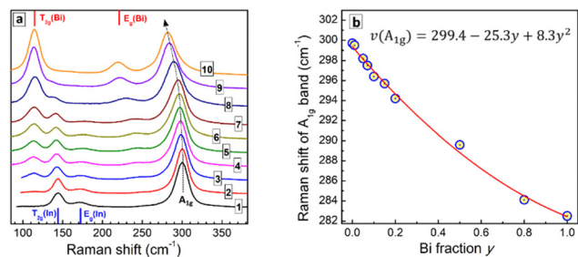
Fig. 6 (a) Raman spectra of CANBIC perovskites with varied Bi fraction \gamma = 0 (1), 0.01 (2), 0.05 (3), 0.07 (4), 0.10 (5), 0.15 (6), 0.20 (7), 0.50 (8), 0.80 (9), and 1.00 (10). (b) Frequency of the A_{1g} mode as a function of Bi fraction \gamma (scatter). Solid red line represents the best fit with a polynomial function " \nu(A_{1g}) versus \gamma " presented in the figure.
