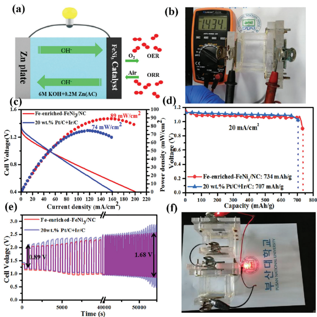
Fig. 11 (a) A schematic illustration of the home-made Zn–air battery. (b) OCV of the as-assembled Zn–air battery with an Fe-enriched-FeNi 3 /NC air-cathode. (c) The discharge polarization curves and the corresponding power density curves of the battery with Fe-enriched-FeNi 3 /NC and 20 wt.% Pt/C + Ir/C air-electrodes, respectively. (d) Specific capacity plots of Fe-enriched-FeNi 3 /NC and 20 wt.% Pt/C + Ir/C based Zn–air batteries tested at 20 mA cm −2 . (e) Galvanostatic discharge–charge cycling curves of Fe-enriched-FeNi 3 /NC and 20 wt.% Pt/C + Ir/C based batteries at a current density of 10 mA cm −2 , respectively. (f) Photograph of a red LED lightened by two series-connected liquid Zn–air batteries with an Fe-rich-FeNi 3 /NC air-cathode. Reproduced from ref. 260 with permission from Elsevier Inc.
