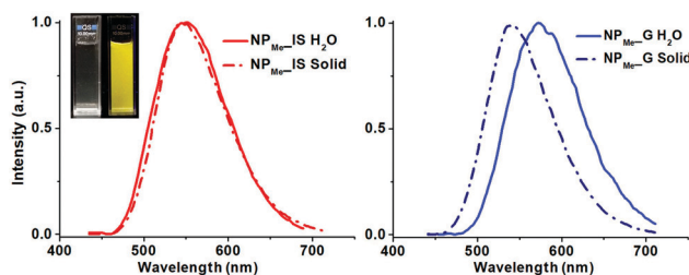
Fig. 4 Emission spectra at room temperature of NP_{Me-IS} (left, red) and NP_{Me-G} (right, blue) in the solid state (dotted line) and in water suspension (solid line). Inset: photograph of the aqueous suspension of NP_{Me-IS} under visible and UV \lambda_{exc} 370 nm illumination.
