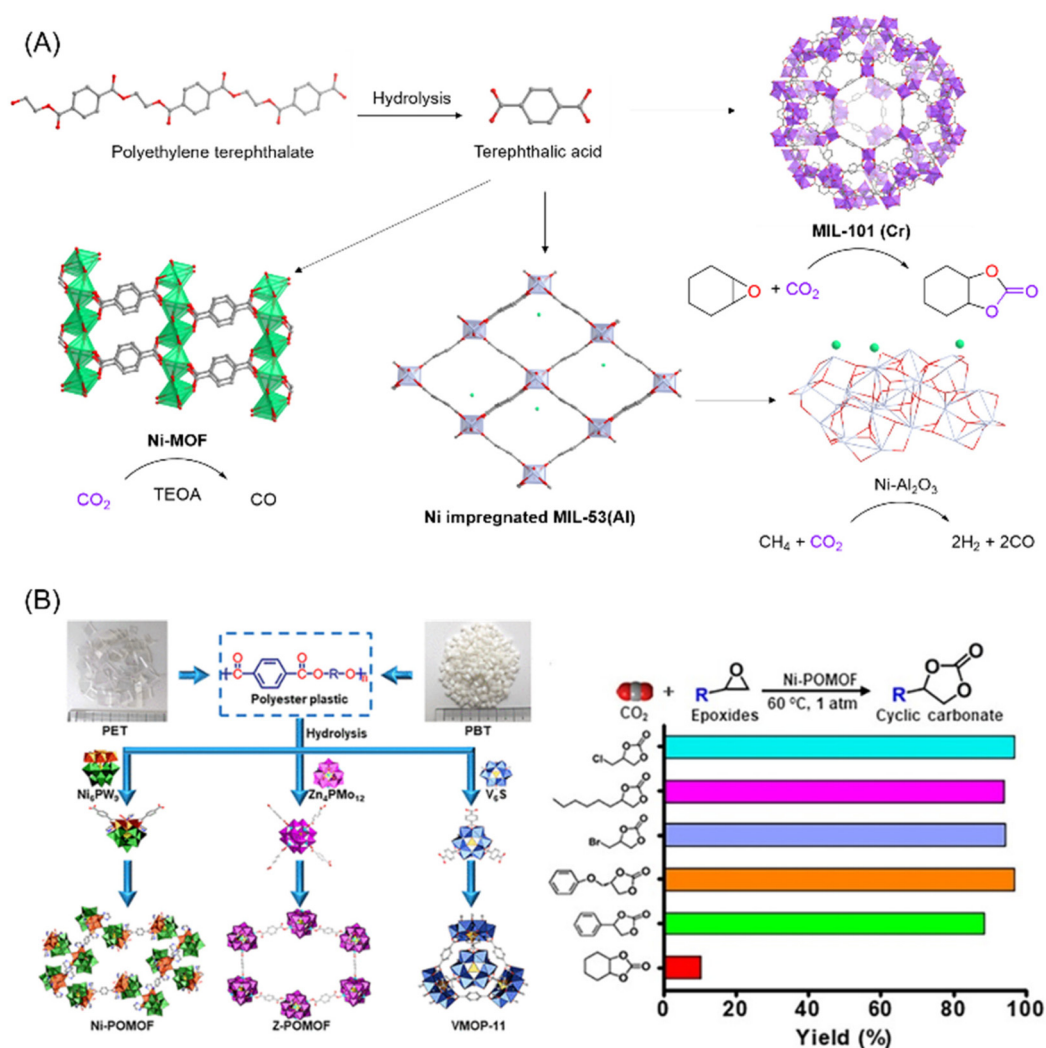
Fig. 4 (A) Schematic illustration of the various routes for transforming PET into MOFs, and the catalytic activity of the MOFs for the utilization of \text{CO}_2 , figures generated from published CIF files. 84–86 (B) Conversion of PET/PBT into POMOFs and catalytic performance of the Ni-POMOF for \text{CO}_2 utilisation into cyclic carbonates. This figure has been published in CCS Chemistry 2019; "Polyoxometalate-Induced Efficient Recycling of Waste Polyester Plastics into Metal–Organic Frameworks", 83 and is available online at 10.31635/ccschem.019.20190028 ( https://www.chinesechemsoc.org/doi/10.31635/ccschem.019.20190028 ).
