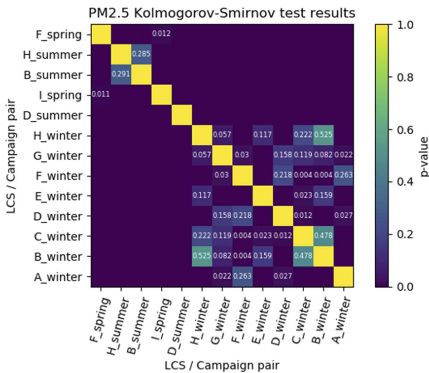
Fig. 6 Results of the Kolmogorov–Smirnov test for the PM_{2.5} calibrations. The color scale in the plots indicates the p -values from the tests. Only the p -values which indicate an origin from the same distribution ( p -value > 0.05, with a subsequent Bonferroni correction) are written on the plot.
