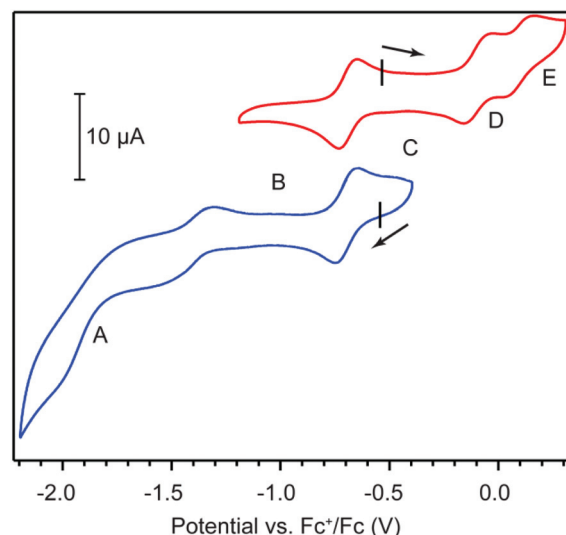
Fig. 2 Cyclic voltammograms of 1 in a 0.15 M solution of TBAPF 6 in THF under \text{N}_2 . Black tick marks indicate open circuit potentials. A, B, C, D, and E mark, respectively, the dominant species within the [\text{Ni}_3(\text{HITP}^{n-})] series ( n = 5, 4, 3, 2, 1 ).
