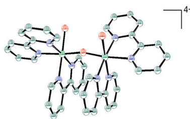
Fig. 118 Molecular structure of cis,cis - [(\text{bpy})_2\text{Ru}(\text{H}_2\text{O})\text{Ru}^{\text{III}}(\text{OH}_2)-(\text{bpy})_2]^{4+} ( 1 ). 1477 Reprinted with permission from ref. 1477 Copyright 1985. American Chemical Society.
