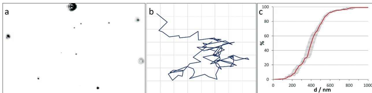
Fig. 2 a) An example of a colour-inverted still frame obtained by NTA, showing scattering species as dark points; b) an example of a trajectory of a scatterer tracked by NTA; c) an example of a cumulative cluster size distribution obtained from averaged NTA runs.
