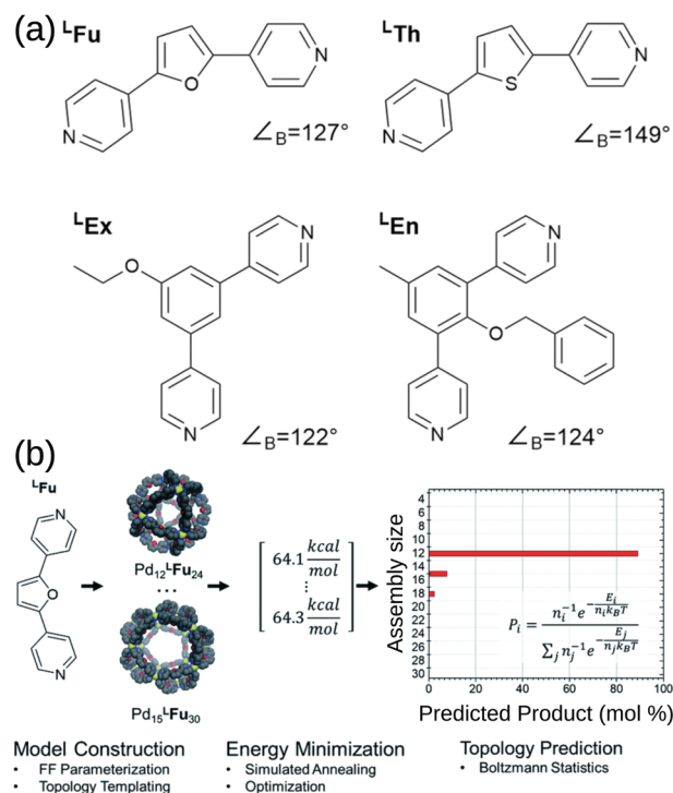
Fig. 7 (a) Structures of the bipyridyl linker molecules used in this study. Bond angles, \angle_B , are estimated from B3LYP/def2-TZV minimized structures. (b) Flow chart for topological prediction of homoleptic assemblies featuring the formation of homoleptic \text{Pd}_n\text{L}_{2n} assemblies. The linker structure is used to construct a library of possible assembly outcomes, which are subjected to a simulated annealing and structural optimization procedure using implicit solvation. The resulting minimum energies, E , are treated as microstates, and the topological distribution is determined using Boltzmann statistics with a weighting factor ‘ n ’ corresponding to the number of linker components in the assembly. Reprinted with permission from ref. 114.
