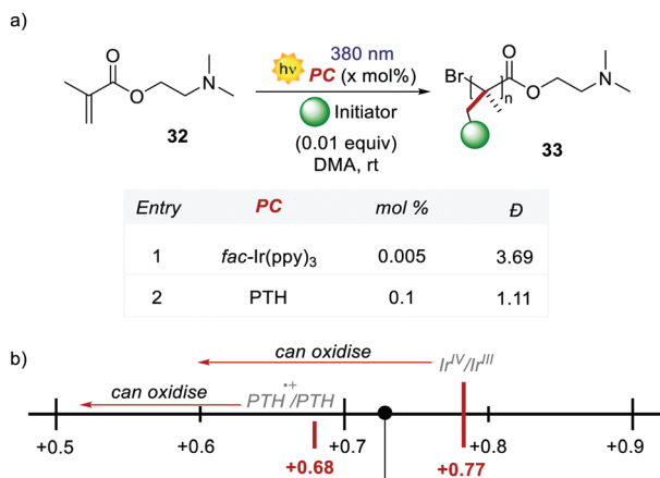
Scheme 18 (a) Polymerisation of dimethylaminoethyl methyl methacrylate. Comparison between the performances of PTH and fac -Ir(ppy) 3 . (b) Graphical depiction of the oxidation potentials (vs. SCE in MeCN) of 32 , PTH and fac -Ir(ppy) 3 .
