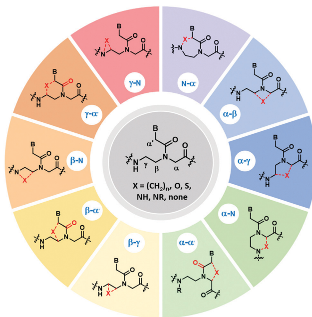
Fig. 13 Possible sites for modification of aegPNA by forming a cyclic structure as part of the backbones.
