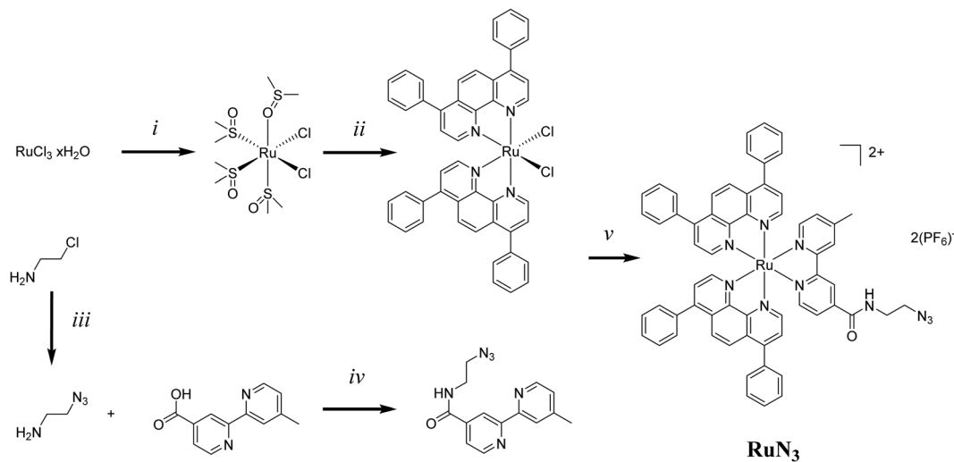
Fig. 2 Synthetic procedure for RuN 3 ; (i) EtOH/DMSO, reflux, 4 h; DMSO, 125 °C, 1 h, 85%; (ii) Bphen, LiCl, DMF, reflux, 5 h, 72%; (iii) \text{NaN}_3 , \text{H}_2\text{O} , 80 °C, 12 h, 82%; (iv) EDCl, NHS, DIPEA, \text{CH}_2\text{Cl}_2 , r.t., 12 h, 56%; (v) MeOH, \text{H}_2\text{O} , reflux, 15 h, 64%.
