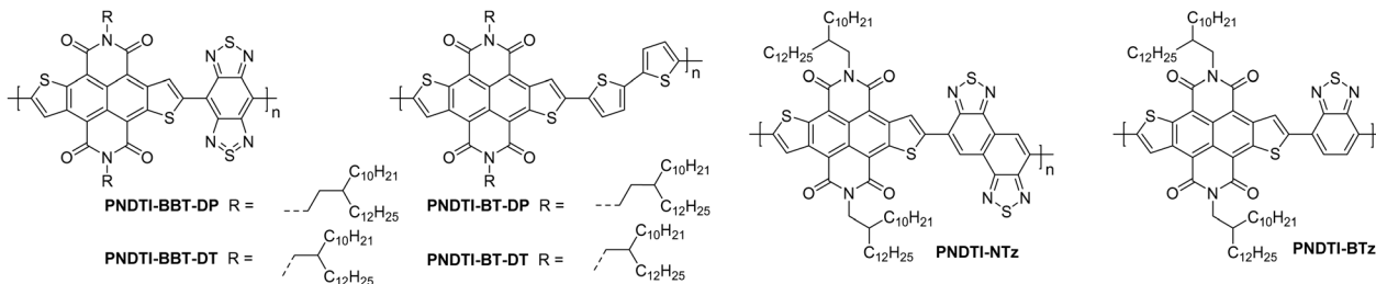
Fig. 7 Chemical structures of reported OTFT polymeric materials containing NDTI derivatives, including their published synonyms.
