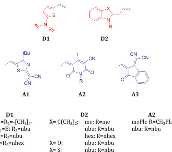
Fig. 1 Molecular structures of the donor and acceptor units constituting the library of mercocyanines investigated in the current work. Details of the various side chains and heteroatoms characterising the D and A units are reported at the bottom.
