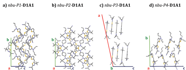
Fig. 5 Crystal structures (supercell) of nbu-Pn-D1A1 polymorphs as obtained in the current work, namely (a) nbu-P1-D1A1 (chloroform, XRD at room temperature), (b) nbu-P2-D1A1 (chloroform, XRD at 100 K), (c) nbu-P3-D1A1 (mesitylene, XRD at 100K); (d) nbu-P4-D1A1 as reported in ref. 28.
