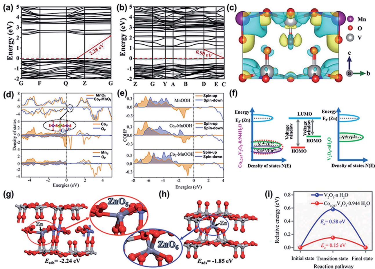
Fig. 2 (a and b) Calculated total band structures and electron density difference of pure \text{V}_2\text{O}_5 and \text{Mn}^{2+} -doped \text{V}_2\text{O}_5 . (c) Electron density difference of \text{Mn}^{2+} -doped \text{V}_2\text{O}_5 . (a–c) Reproduced with permission. 57 Copyright 2019, Wiley-VCH. (d) DOS of \text{MnO}_2 and \text{Co}^{4+}-\delta\text{-MnO}_2 . (e) COHP of \text{MnO}_6 (the c -axis) at different positions of \text{MnOOH} . (d and e) Reproduced with permission. 70 Copyright 2020, Wiley-VCH. (f) Schematic illustration of the energy versus DOS in \text{Co}_{0.247}\text{V}_2\text{O}_5 \cdot 0.944\text{H}_2\text{O} and \text{V}_2\text{O}_5 \cdot n\text{H}_2\text{O} cathodes. (g and h) The optimized configuration of Zn-adsorbed \text{Co}_{0.247}\text{V}_2\text{O}_5 \cdot 0.944\text{H}_2\text{O} and \text{V}_2\text{O}_5 \cdot n\text{H}_2\text{O} frameworks, respectively, and their corresponding adsorption energies. The gray spheres represent adsorbed Zn atoms, and Co atoms are depicted as blue spheres. (i) The diffusion energy barrier profiles of \text{Co}_{0.247}\text{V}_2\text{O}_5 \cdot 0.944\text{H}_2\text{O} and \text{V}_2\text{O}_5 \cdot n\text{H}_2\text{O} . (f–i) Reproduced with permission. 58 Copyright 2019, Wiley-VCH.
