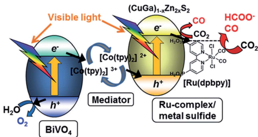
Scheme 20 Schematic diagram of the Z-schematic system for CO 2 reduction consisting of the MC55 modified (CuGa) 1-x Zn 2x S 2 hybrid photocatalyst, a BiVO 4 photocatalyst, and a [Co(tpy) 2 ] 3+/2+ redox shuttle electron mediator. Reproduced with permission from ref. 127, Copyright 2018, Royal Society of Chemistry.
