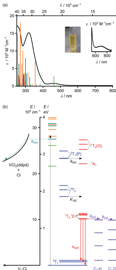
Fig. 1 (a) Absorption spectrum including a zoom into the red spectral region (black) and photograph of \text{VCl}_3(\text{ddpd-}[D_0]) in \text{CH}_3\text{CN} . The vertical bars correspond to spin-allowed CT transitions calculated by TDDFT-UKS (hypsochromically shifted by 3400 \text{cm}^{-1} ). The colour code of the vertical bars indicates the major character of the transition as ddpd \rightarrow V ^3\text{LMCT} (light green), Cl \rightarrow V ^3\text{LMCT} (petrol green), ILCT (orange) and V \rightarrow ddpd ^3\text{MLCT} (purple). (b) Jablonski diagram constructed from TDDFT-UKS (ddpd \rightarrow V ^3\text{LMCT} (light green), Cl \rightarrow V ^3\text{LMCT} (petrol green) and ILCT (orange)) and CASSCF-NEVPT2 calculations ( ^3\text{MC} states in blue; ^1\text{MC} states in red). Notation of MC states is according to octahedral symmetry. ISC = intersystem crossing; diss = V–Cl homolysis; NIR = NIR emission; C–H and C–D overtones in purple = multiphonon relaxation (experimental overtone energies from ref. 34).
