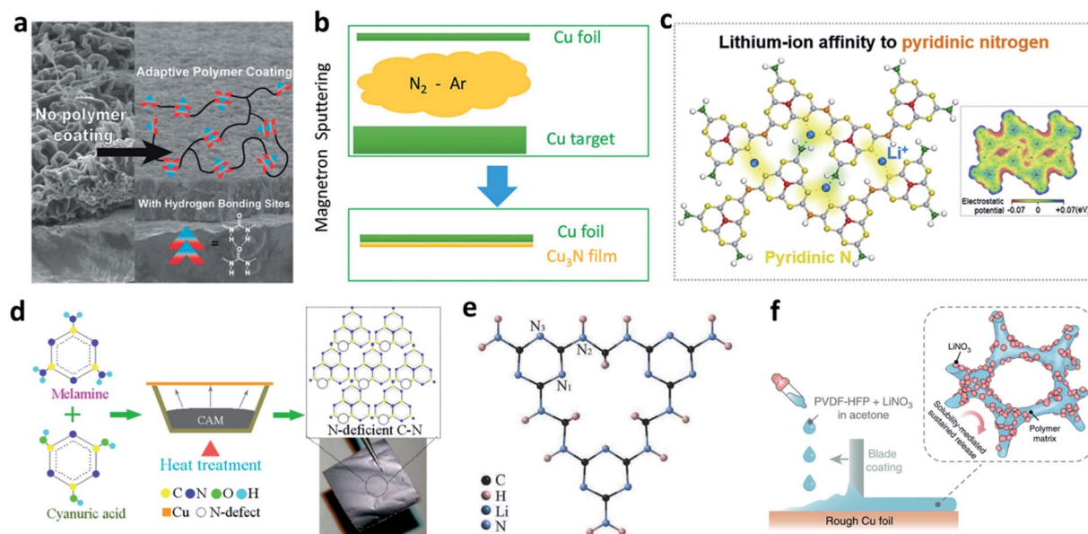
Fig. 12 Modification of a Cu substrate with nitrided interfaces. (a) SEM images showing the effect of an adaptive polymer coated on Cu foil to suppress Li dendrite growth, and the structure of the adaptive polymer layer; 123 reproduced with permission. Copyright 2016, American Chemical Society. (b) Schematic illustration of the preparation of a \text{Cu}_3\text{N} layer on Cu foil by using the reaction of Cu and \text{N}_2 gas; 124 reproduced with permission. Copyright 2018, American Chemical Society. (c) Illustration of the pyridinic nitrogen in \text{g-C}_3\text{N}_4 , which serves as a \text{Li}^+ affinity centre; 125 reproduced with permission. Copyright 2020, Elsevier. (d) Preparation of a defect-rich C–N polymer on Cu foil; 126 reproduced with permission. Copyright 2020, American Chemical Society. (e) Structure of the poly-melamine-formaldehyde framework; 127 reproduced with permission. Copyright 2018, John Wiley and Sons. (f) Schematic illustration of blade coating of a PVDF-HFP + \text{LiNO}_3 layer on rough Cu foil. 128 Reproduced with permission. Copyright 2018, Springer Nature.
