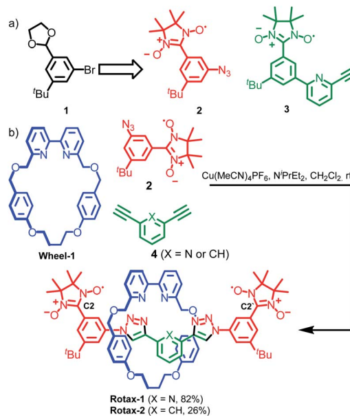
Scheme 1 (a) Protected 3-bromo-5- tert -butylbenzaldehyde starting material used in the synthesis of nitronyl nitroxide based half-axles 2 and 3 (used in the synthesis of Rotax-3, vide infra ). (b) Synthesis of spin-labelled rotaxanes Rotax-1 and Rotax-2. The structures of corresponding axles, Axle-1 and Axle-2 are identical with the omission of the macrocycle.
