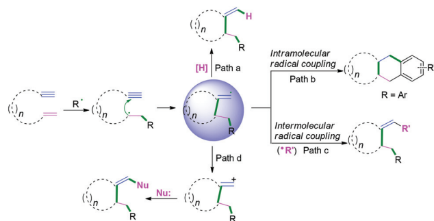
Scheme 13 Plausible mechanism of radical cyclization to 1,n-enynes.
