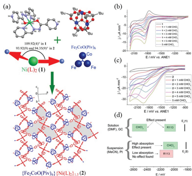
Fig. 7 A Fe^{III} – Ni^{II} bimetallic coordination polymer as a dehalogenation electrocatalyst: (a) synthesis scheme and structures, (b) CV curves of the Ni^{II} metalloligand in DMF with the addition of CHCl_3 , (c) CV curves of the suspension containing the Fe^{III} – Ni^{II} bimetallic coordination polymer in CH_3CN with the addition of CHCl_3 , and (d) catalytic activities vs. redox potentials of the catalysts and the halides. Adapted with permission from ref. 102, Copyright 2014 American Chemical Society.
